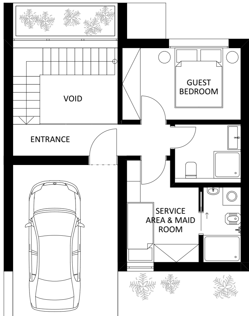
SECOND FLOOR
