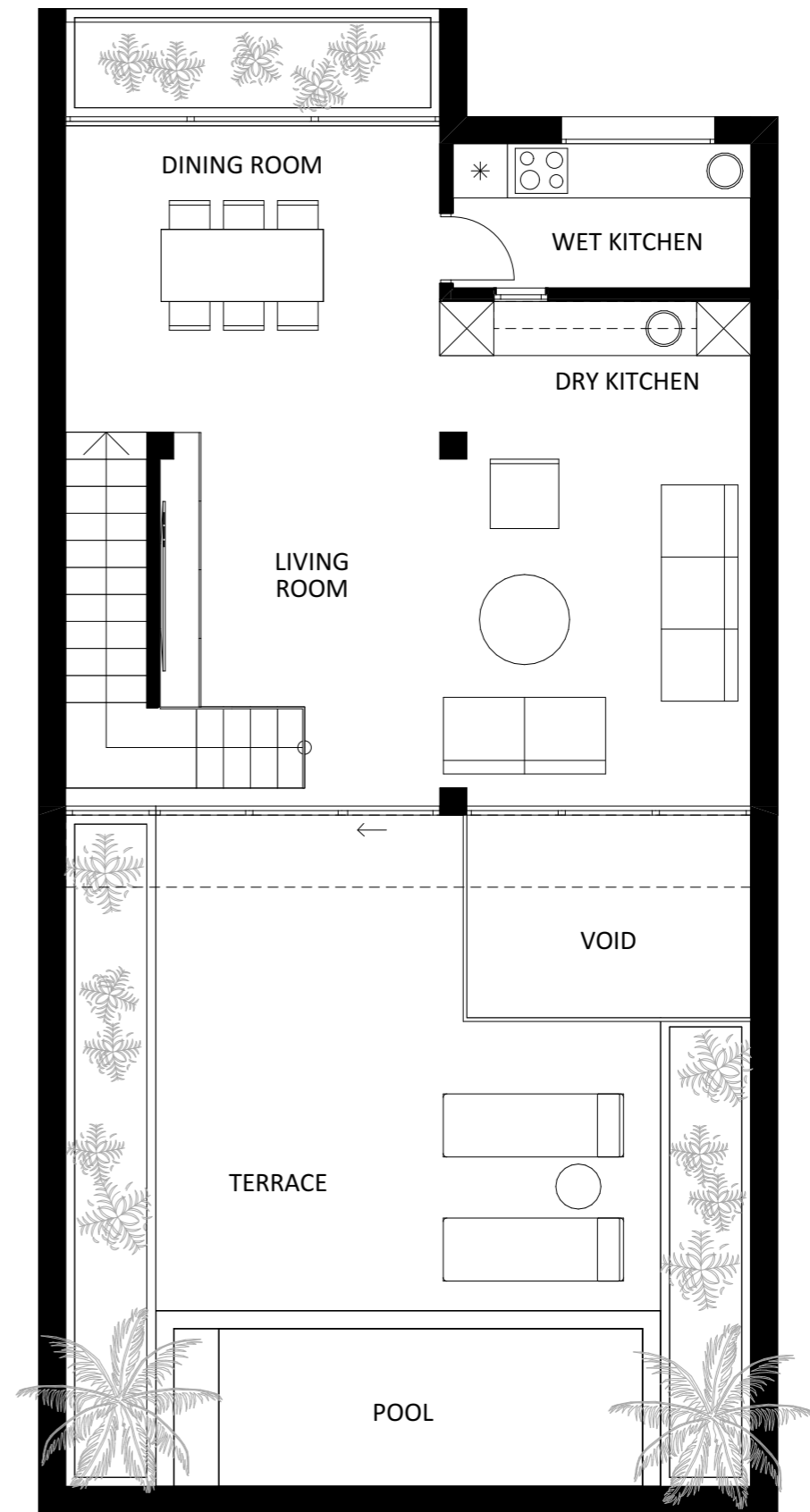
FIRST FLOOR
