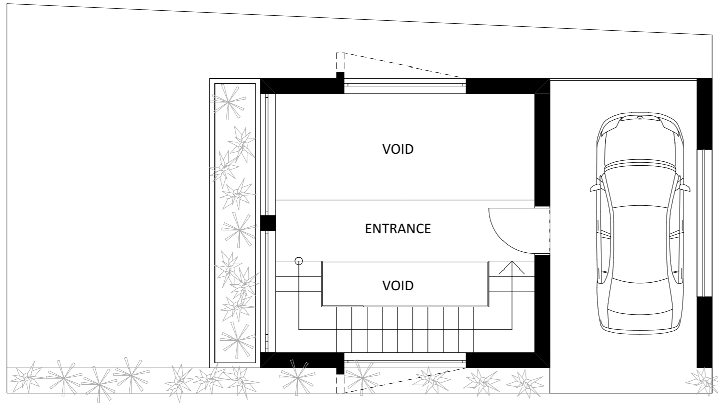
FIRST FLOOR
